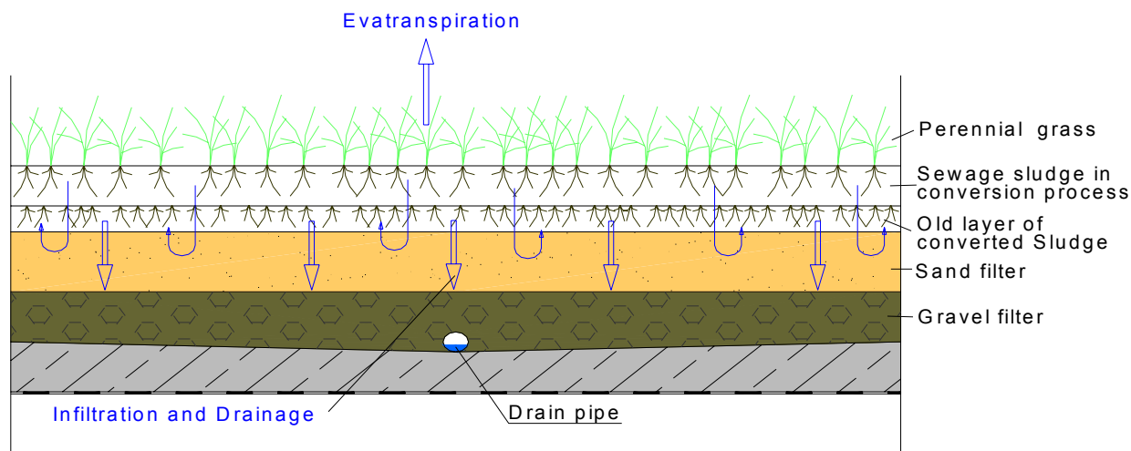
Figure 6: Scheme of a sludge conversion plant (source: ipp Consult )
